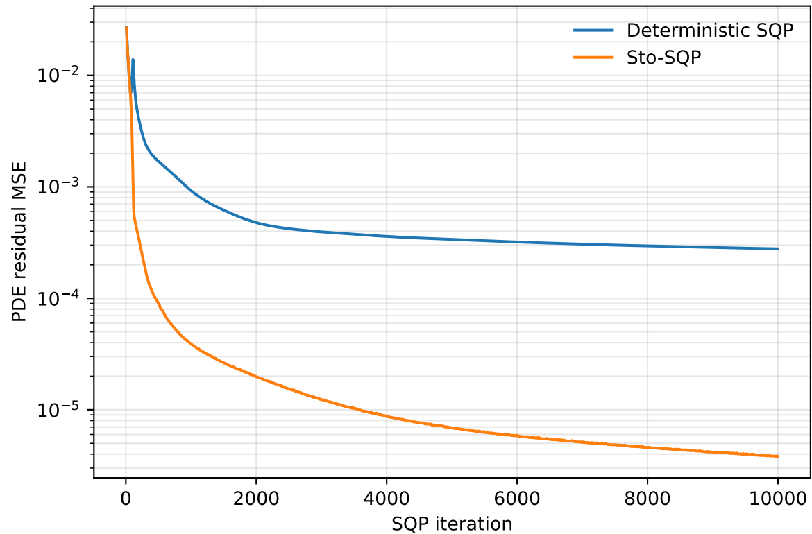
PDE objective
